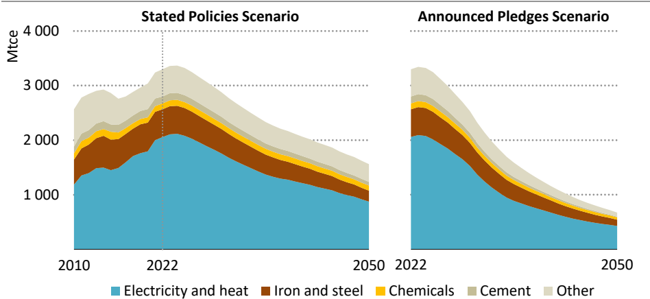
Figure 5.20 ▶ Coal consumption by sector in China by scenario, 2022-2050
