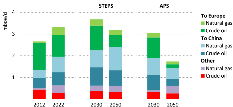
Figure 5.17 ▶ Caspian crude oil and natural gas exports in the STEPS and APS
